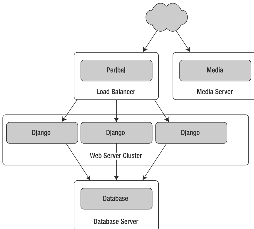
Figure 20-4. A load-balanced, redundant server setup
