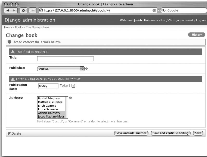
Figure 6-5. An edit form displaying errors
